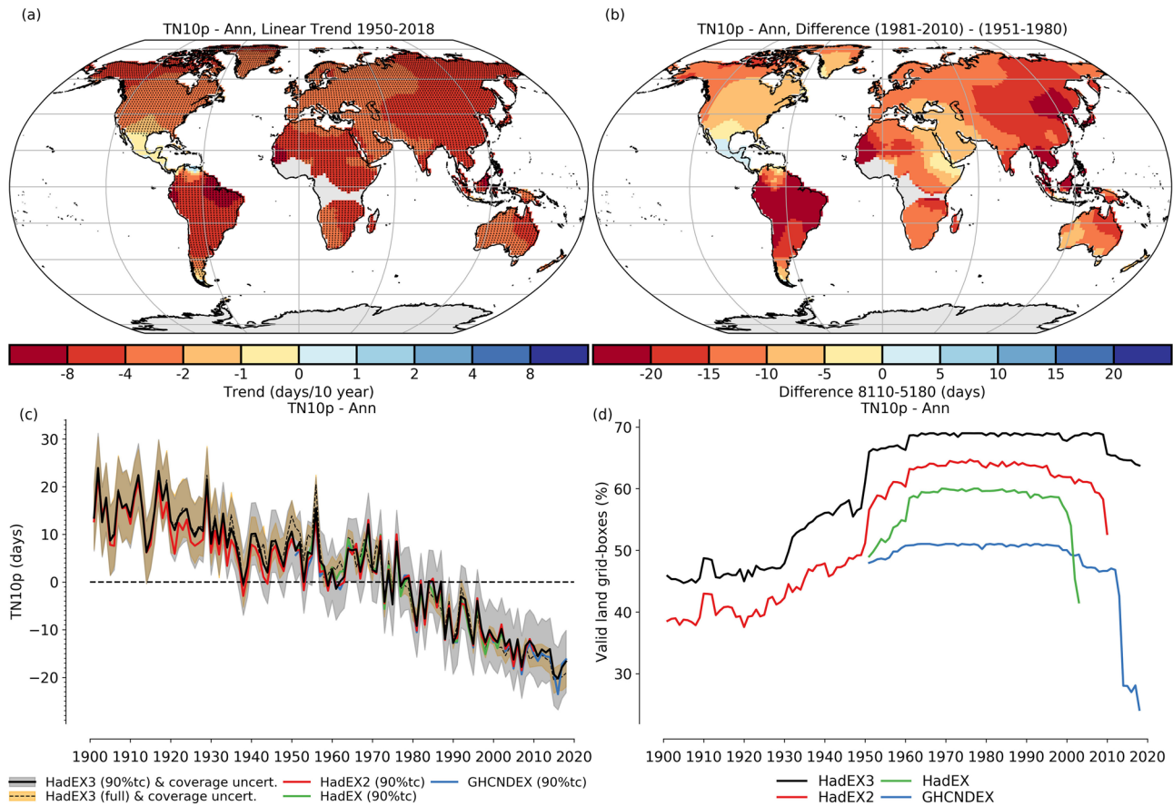
Figure 3. (a) Linear trends in annual series of TN10p over 1950–2018 (days/decade); (b) difference between two 30-year periods (1981–2010 and 1951–1980); (c) time series of HadEX3 compared with HadEX, HadEX2, and GHCNDEX; (d) time series of land fraction containing grid boxes valid data. Details of trend and time series calculation are described in Figure 2. We have converted the units for this index from % into days for clarity.
